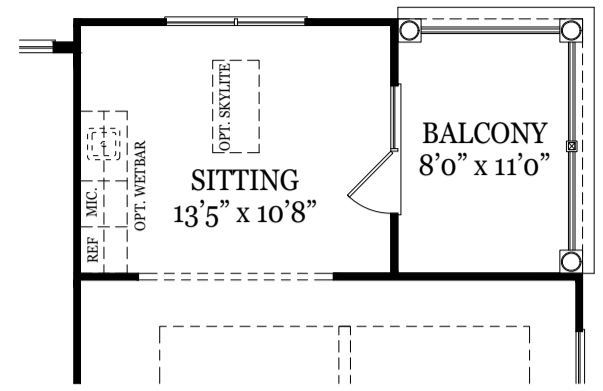
OPT. BALCONY CONDITION
