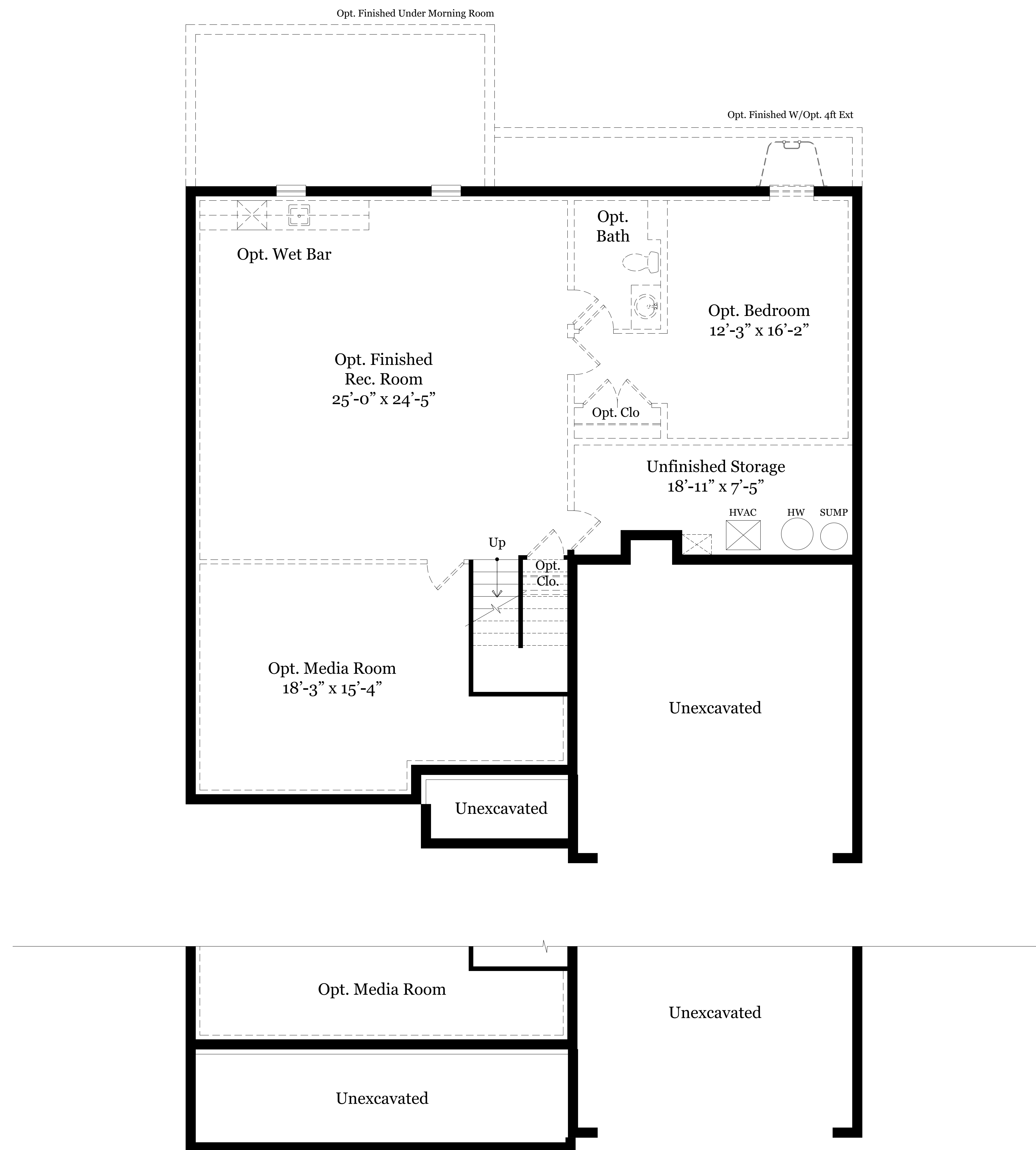
BASEMENT FLOOR PLAN @ ELEVATION B
