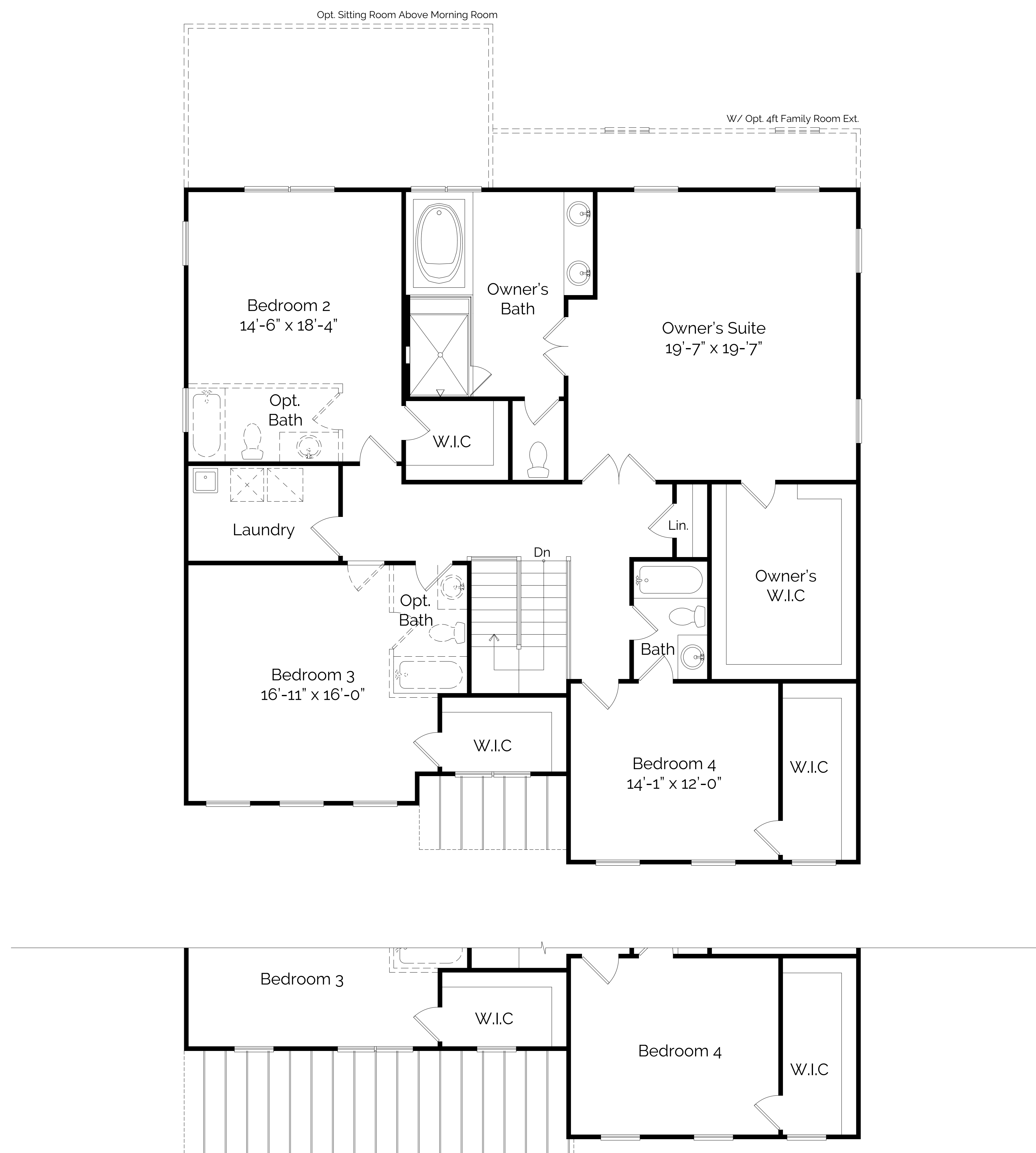
SECOND FLOOR PLAN @ ELEVATION B
