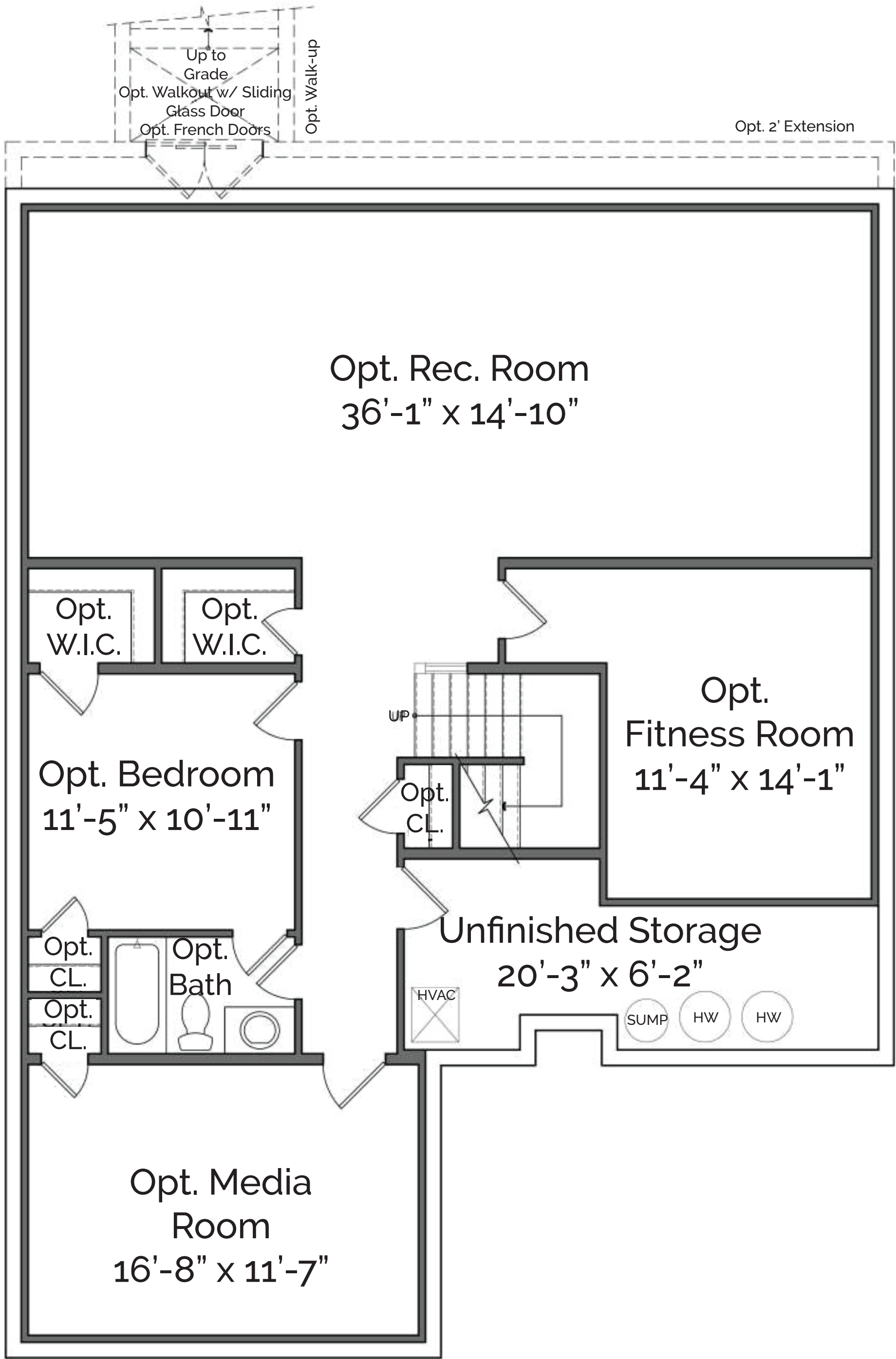
Basement Plan
