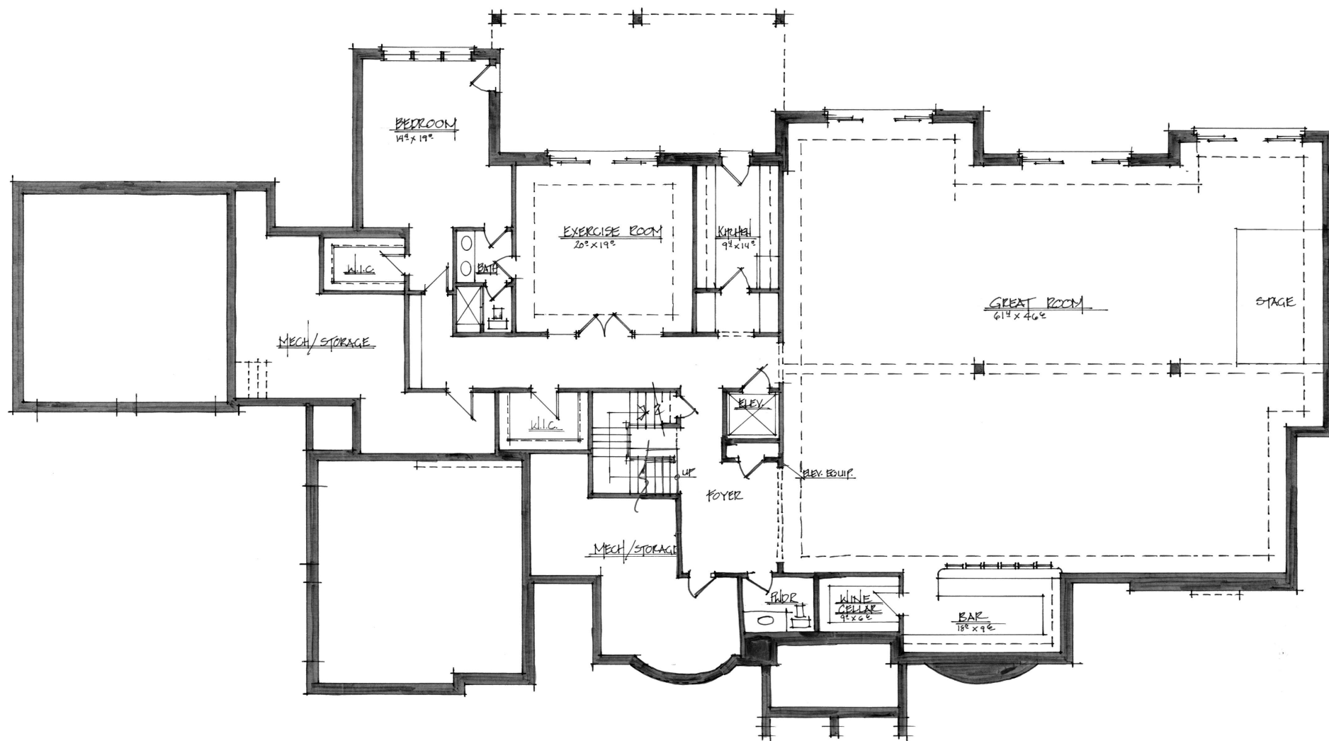
BASEMENT FLOOR PLAN (Optional) FINISHED: 5140.0 S.F.
