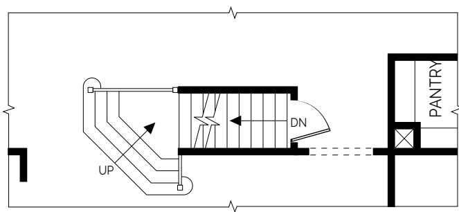
PART. FIRST FLOOR PLAN OPT. FLARED STAIR
