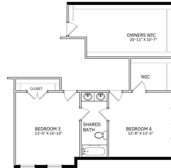
OPT. LAYOUT W/ JACK & JILL BATH
